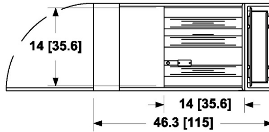
CAD diagram for Model VF35
