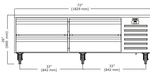
Front (CRB572)
