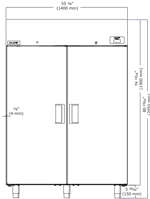
Front (Closed)
