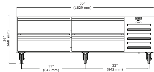
Front (CFB572)
