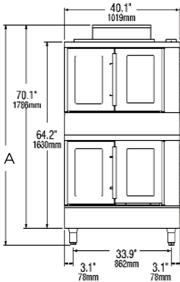
[Front View/Elevation]
