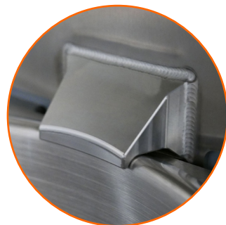
When lifted, the bowl should be fixed underneath the bowl fitting
