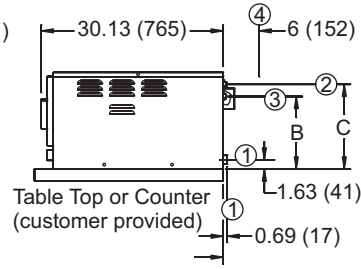
SIDE VIEWS
