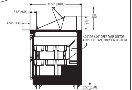
D4472N-18M Right Side View
