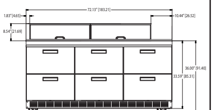
D4472N-24M Elevation View
