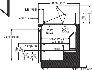
4472N-24M Right Side View
