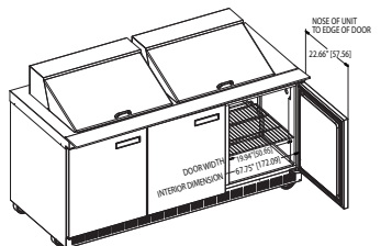
4472N-24M ISO View
