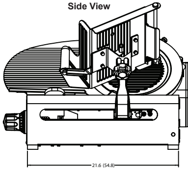
4600N Side View
