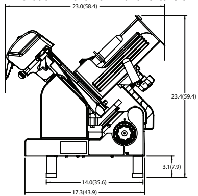
Elevation / Front View with 3" extension legs
