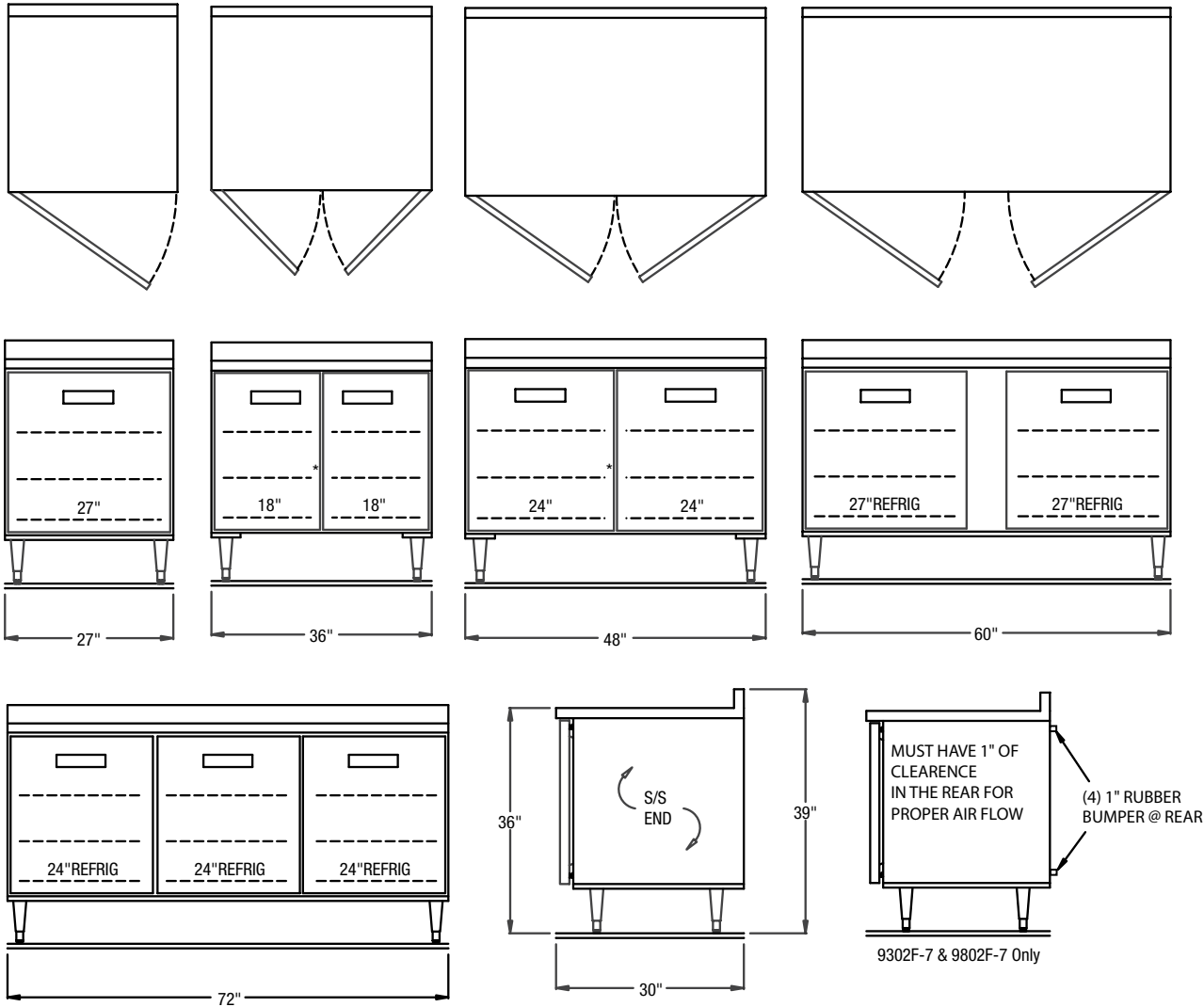
Drawings are to be viewed in the same order as the chart, one drawing to represent refrigerator and freezer units
