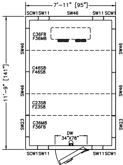
PLAN VIEW RIGHT HINGE SELECT
