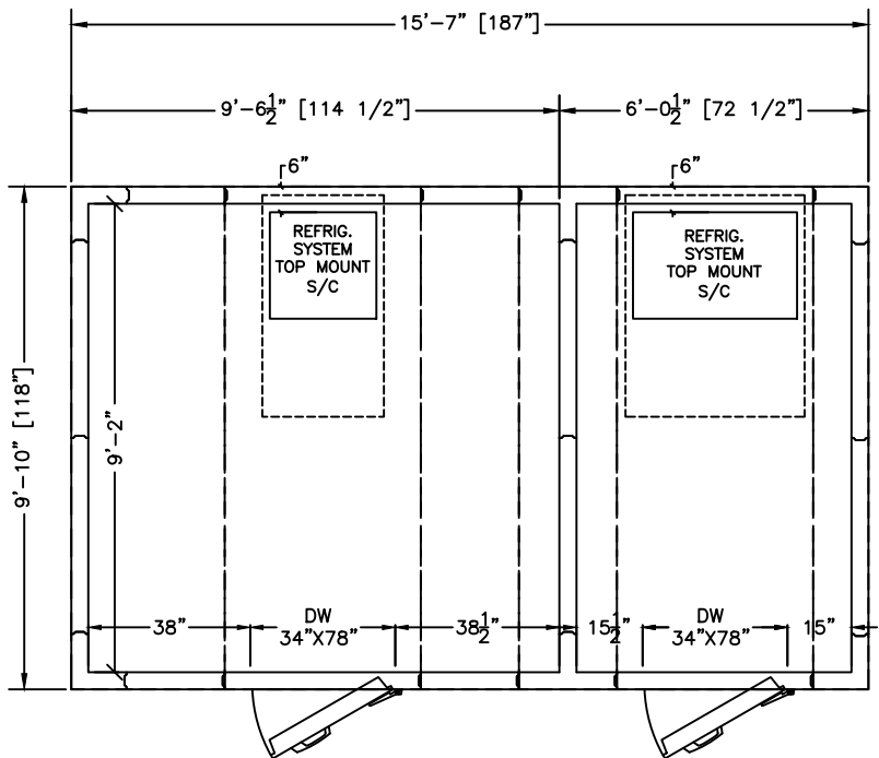
COOLER (WITH FLOOR PANELS)
