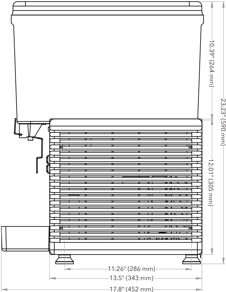
SIDE
