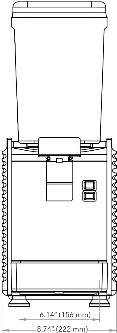
FRONT
