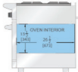
24" and 48" RANGE BASE Larger oven depth accommodates 26" sheet pan front to back.
