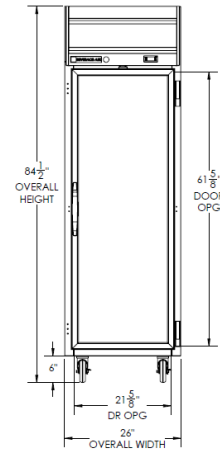
Elevation View
