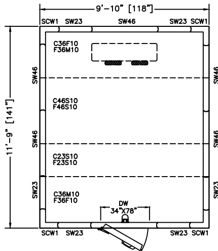
PLAN VIEW
