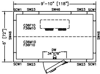
PLAN VIEW RIGHT HINGE SELECT
