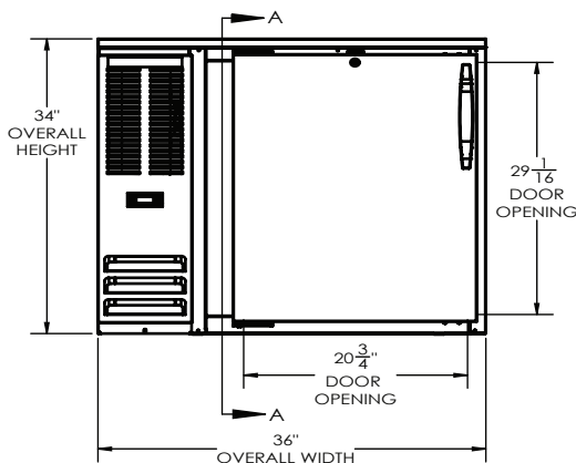
ELEVATION VIEW
