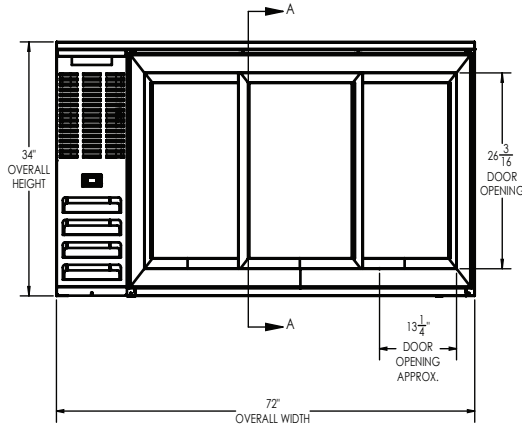
ELEVATION VIEW
