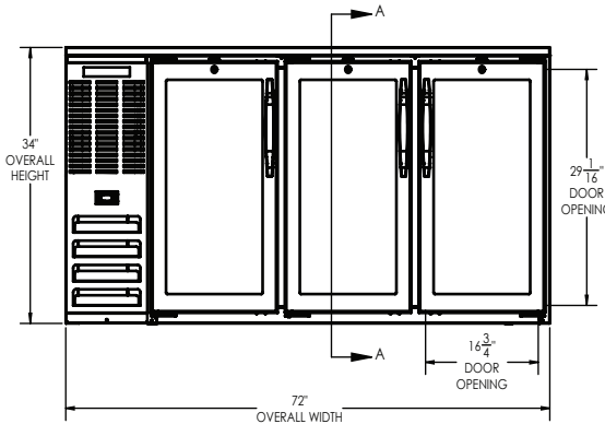
ELEVATION VIEW
