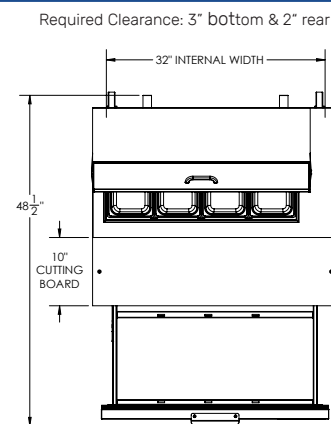
PLAN VIEW
