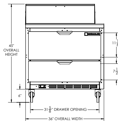
ELEVATION VIEW
