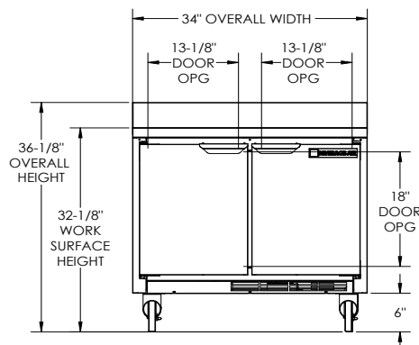
ELEVATION VIEW
