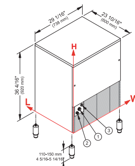
Adjustable feet 4 5/16" – 5 14/16"
