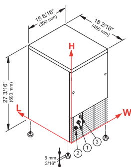
Adjustable feet 3/16"
