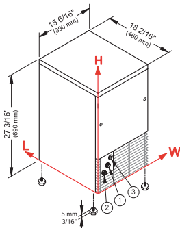
Adjustable feet 3/16"
