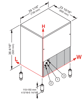
Adjustable feet 4 5/16" – 5 14/16"
