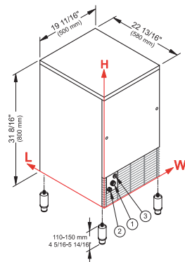
Adjustable feet 4 5/16" – 5 14/16"
