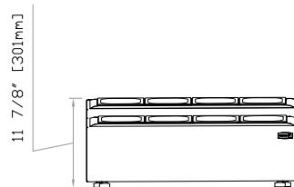
CPR-60-4 Front View
