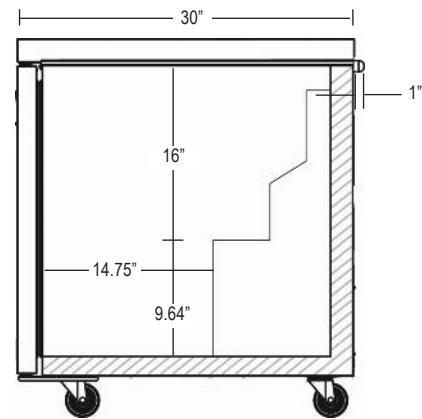
SIDE (Cross Section)
