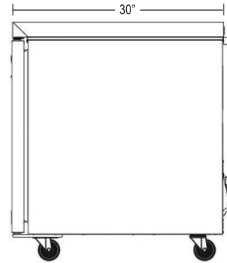
CRMF60 SIDE
