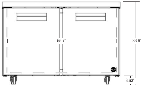
CRMF60 FRONT
