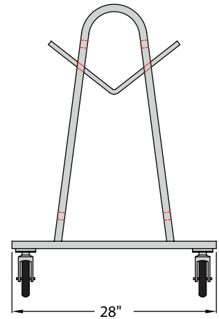
99360 All-Welded Cart
