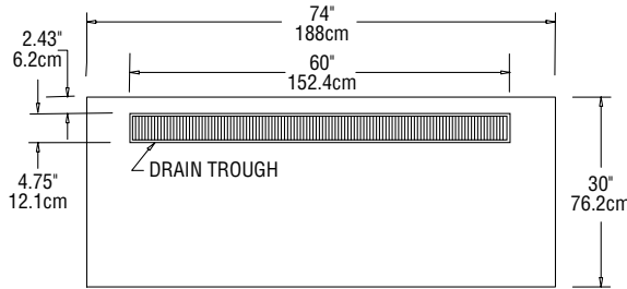
PLAN VIEW SCU-74/ SCU-74-NU
