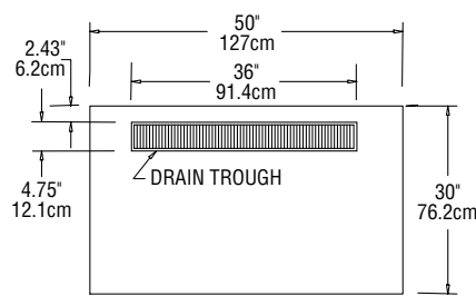
PLAN VIEW SCU-50/ SCU-50-NU
