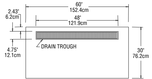
PLAN VIEW SCU-60/ SCU-60-NU
