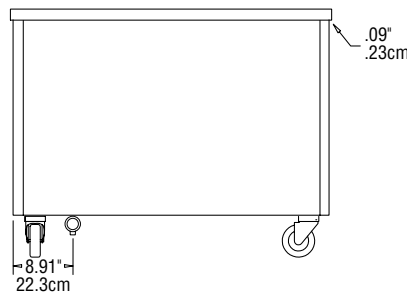
ELEVATION VIEW ALL SCU-NU MODELS
