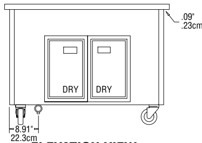
ELEVATION VIEW SCU-50 THROUGH SCU-96 (SCU-96 two compartment not shown)
