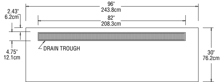
PLAN VIEW SCU-96/ SCU-96-NU
