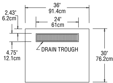
PLAN VIEW SCU-36/ SCU-35-NU
