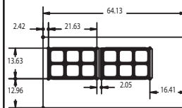
D4464N-12 Pan Cutout Configuration
