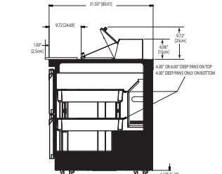
D4464N-12 Right Side View
