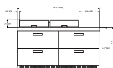
D4464N-12 Elevation View
