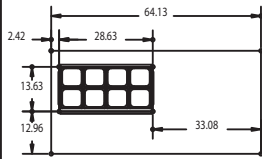
4464N-8 Pan Cutout Configuration
