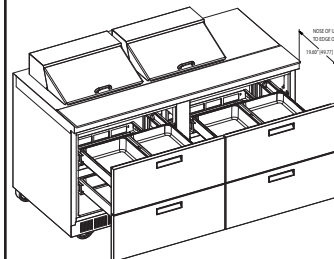
D4464N-12 ISO View
