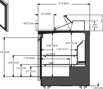
4464N-12 Right Side View
