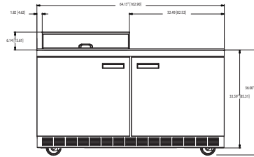
4464N-8 Elevation View
