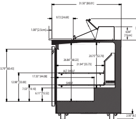
4464N-8 Right Side View
