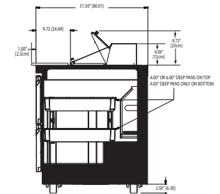
D4464N-8 Right Side View
