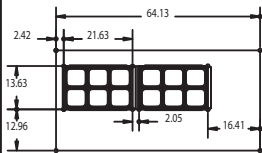
4464N-12 Pan Cutout Configuration
