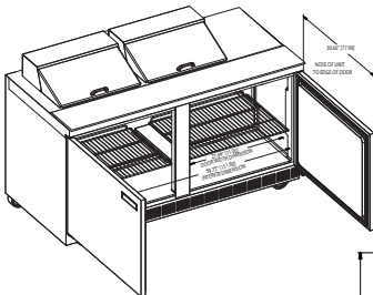
4464N-12 ISO View
