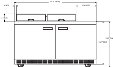
4464N-12 Elevation View
