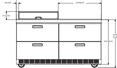
D4464N-8 Elevation View
