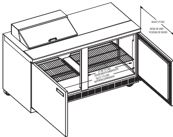
4464N-8 ISO View
