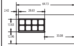
D4464N-8 Pan Cutout Configuration
