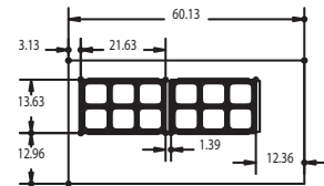
UC4460N-12 Pan Cutout Configuration
