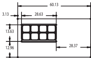
UCD4460N-8 Pan Cutout Configuration
