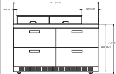
UCD4460N-12 Elevation View
