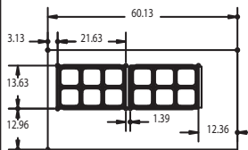
UCD4460N-12 Pan Cutout Configuration
