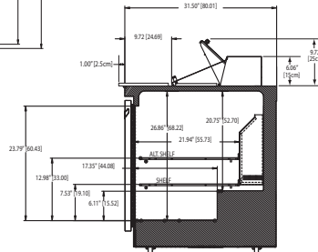
UC4460N-12 Right Side View
