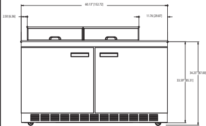
UC4460N-12 Elevation View
