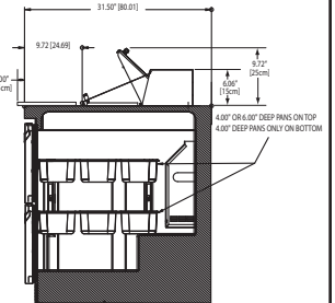
UCD4460N-12 Right Side View
