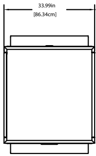
PLAN VIEW ALL 1 SECTION MODELS
