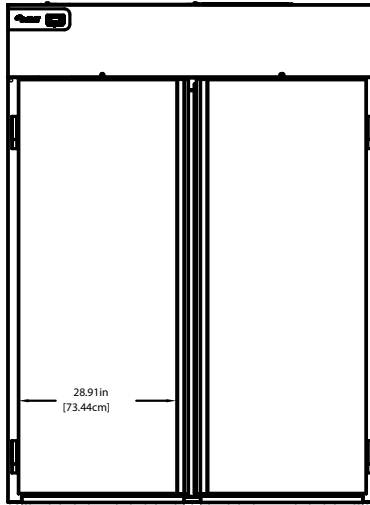
ELEVATION VIEW ALL 2 SECTION MODELS
