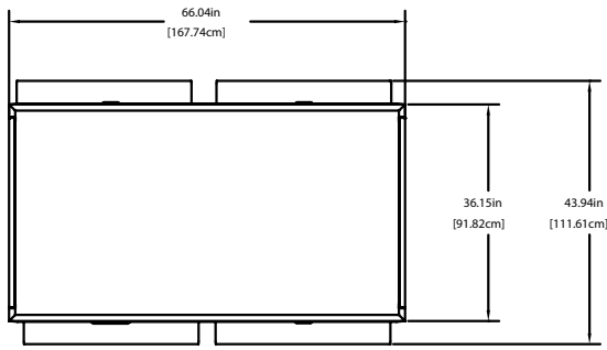
PLAN VIEW ALL 2 SECTION MODELS
