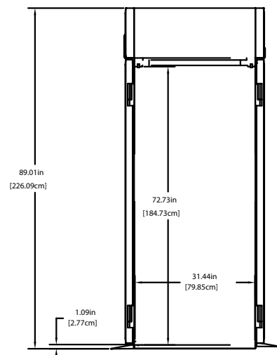
SIDE VIEW ALL MODELS
