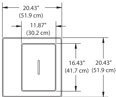
203 Plan View
