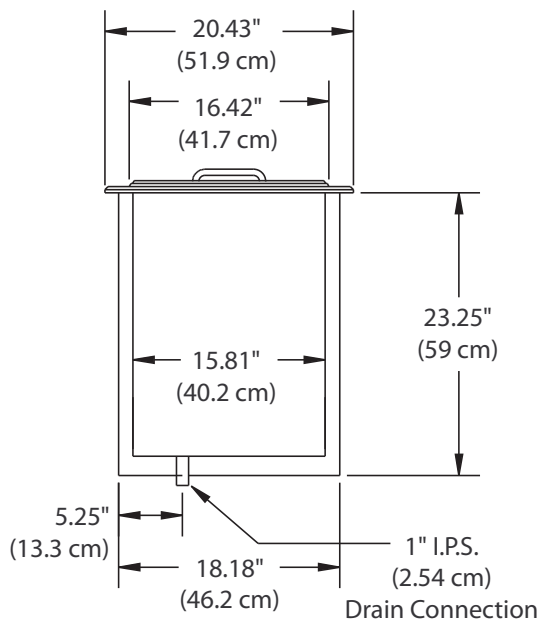
203 Elevation View
