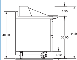
STD4460NP-18M Right Side View
