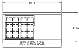
STD4460NP-12M Pan Cutout Configuration
