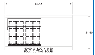
STD4460NP-12M Pan Cutout Configuration
