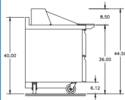
STD4460NP-12M Right Side View
