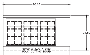
STD4460NP-18M Pan Cutout Configuration
