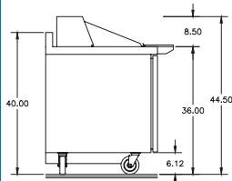
ST4460NP-18M Right Side View
