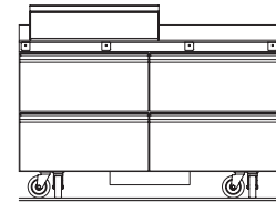
STD4460NP-12M Elevation View
