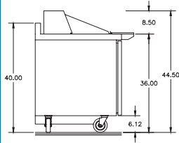
ST4460NP-12M Right Side View
