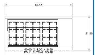
STD4460NP-18M Pan Cutout Configuration
