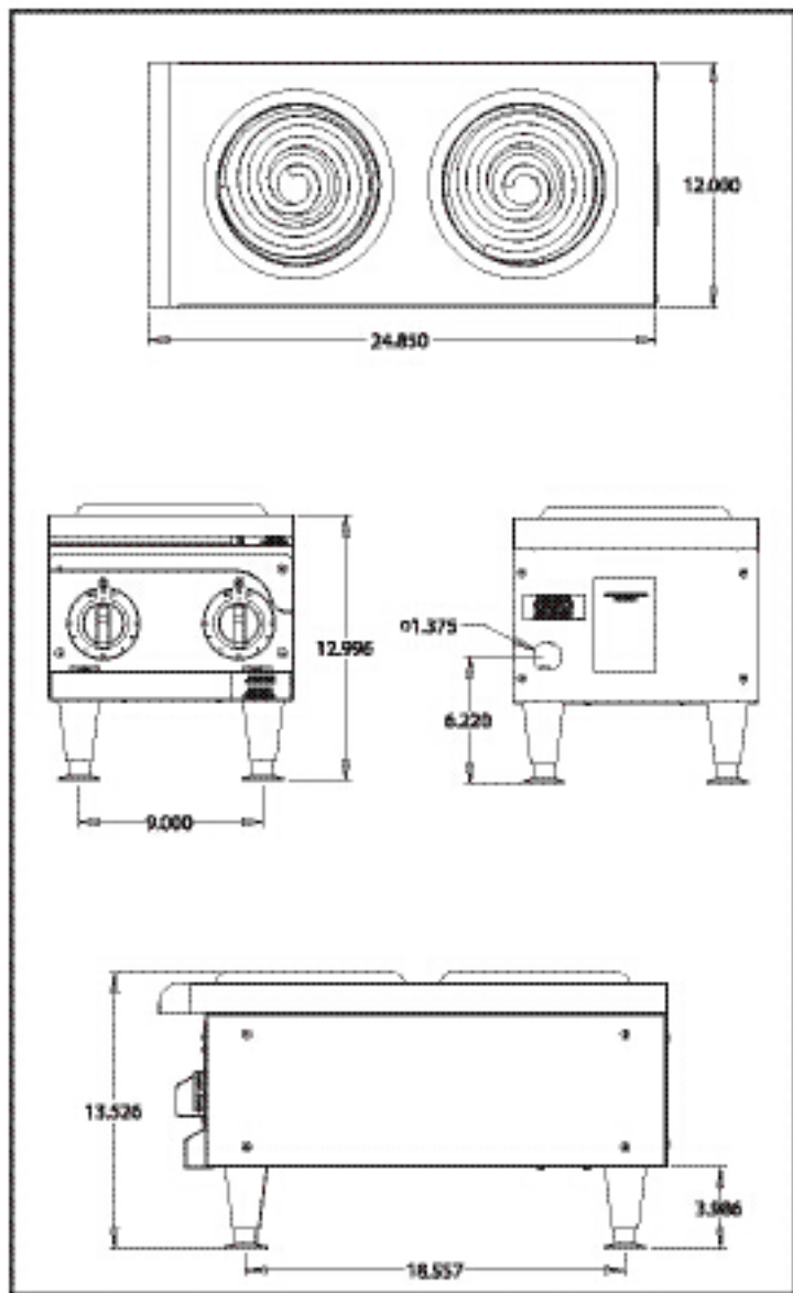
Model EHP, Countertop Electric Hot Plate
