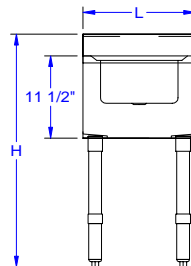
FRONT ELEVATION
