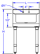
FRONT ELEVATION
