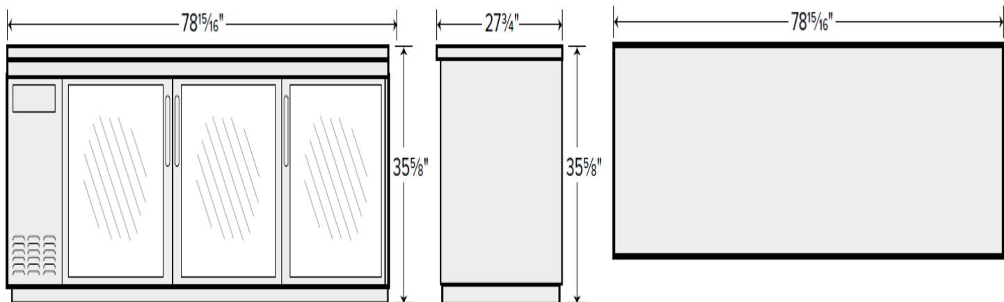
Top View
