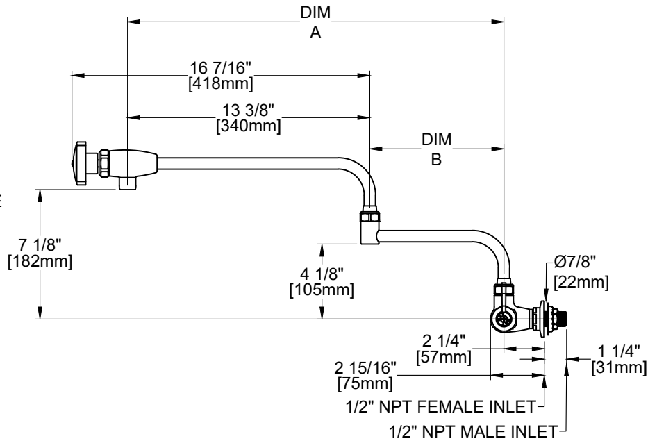
9 3/4" [248mm] QUARTER TURN CERAMIC DISK CARTRIDGE W/ CHECK STEM & COLOR CODED INDEX
