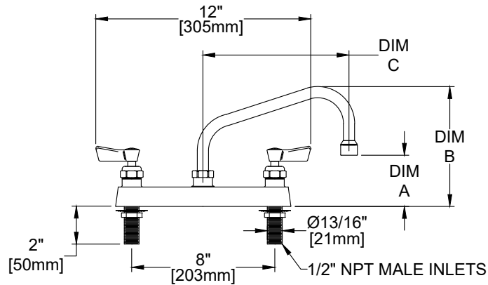
FOOTPRINT
