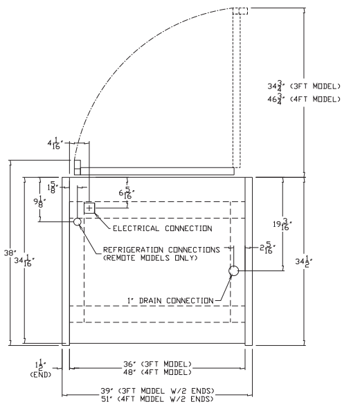
Plan View (3' & 4')
