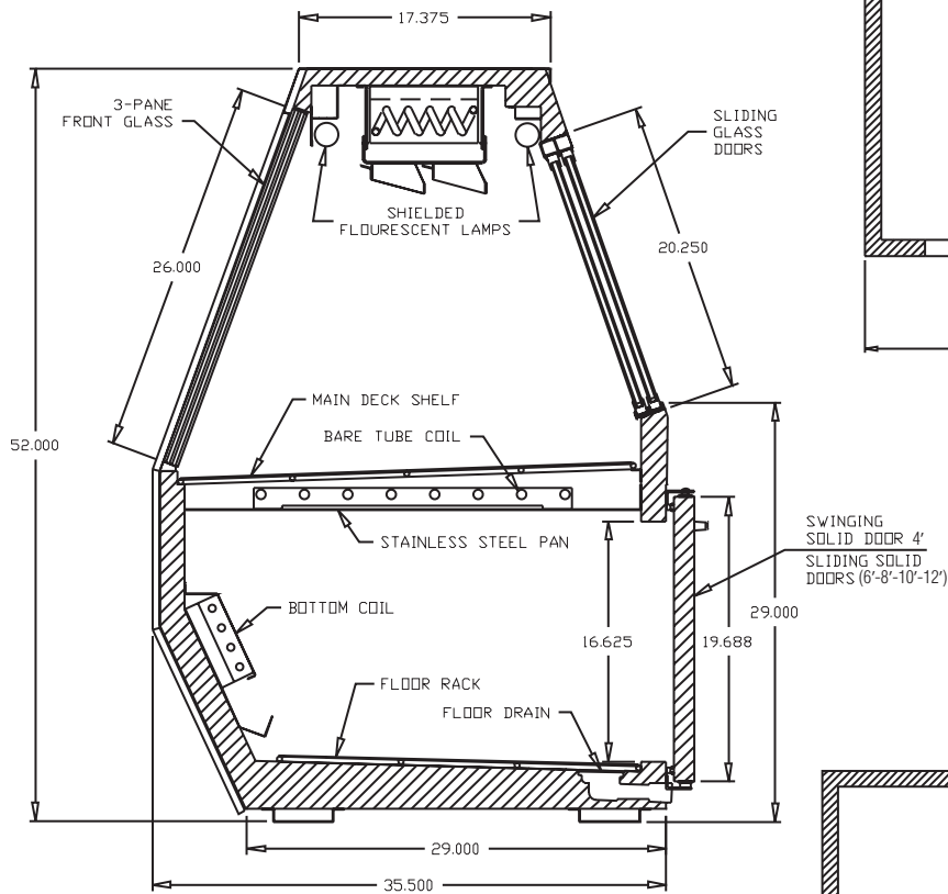
Cross Section
