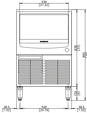
WATER-COOLED
