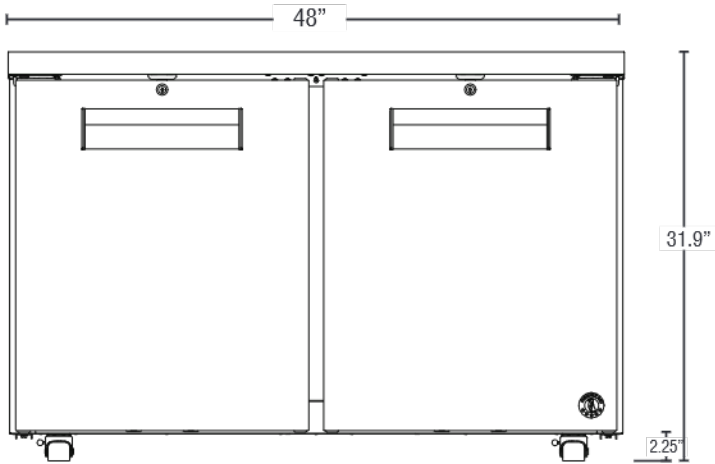
Front view shown with locks (UF48B-LP01)
