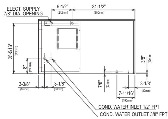
WATER-COOLED UNIT
