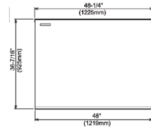
FRONT VIEW - KM-2100/2500
