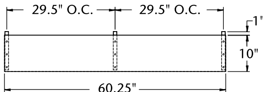
PLAN VIEW MBSP60, MBSMP60, MBUR/MBUF60
