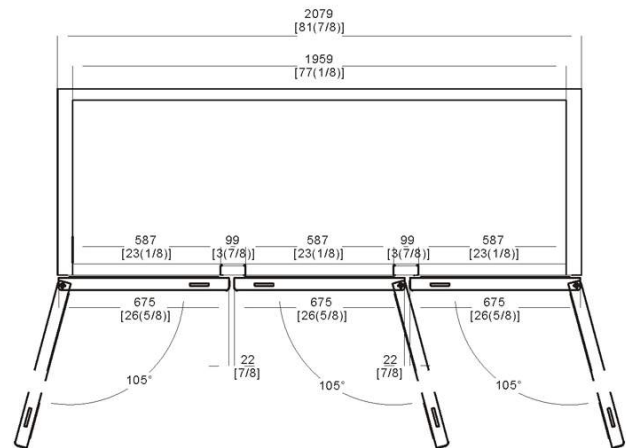
C-72RM TOP VIEW
