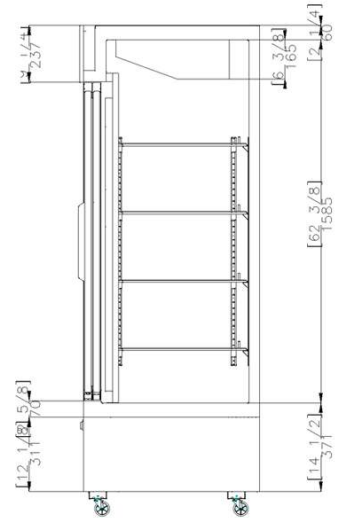
SIDE VIEW ( C-49RS)
