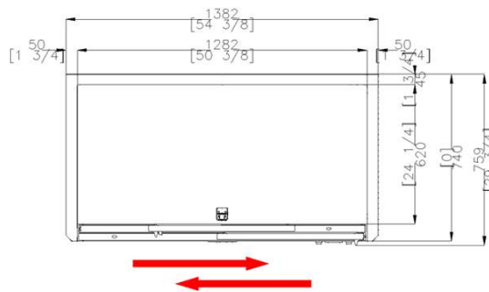
C-49RS TOP VIEW
