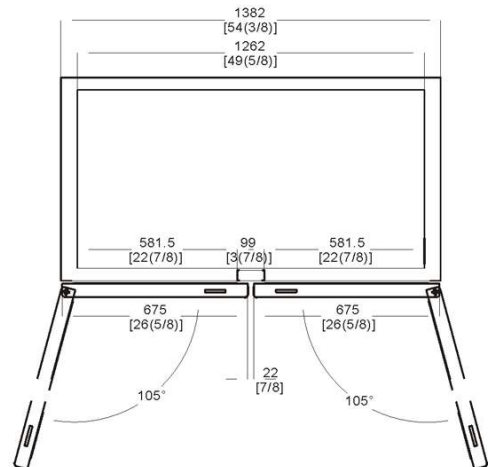
C-49RM TOP VIEW
