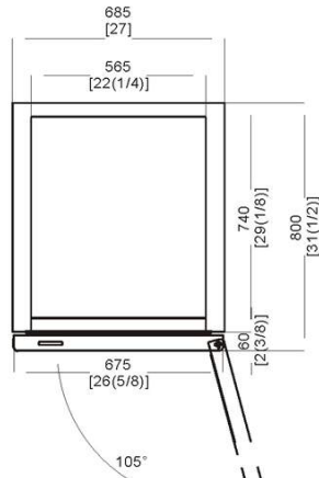
C-23RM TOP VIEW
