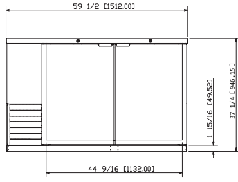
FRONT NLBB59
