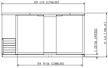
FRONT NLBB69
