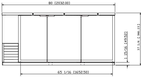
FRONT NLBB79
