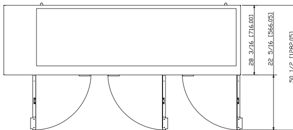
TOP NLBB95
