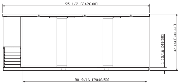
FRONT NLBB95
