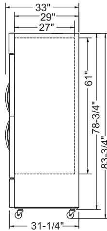
SIDE VIEW ALL MODELS
