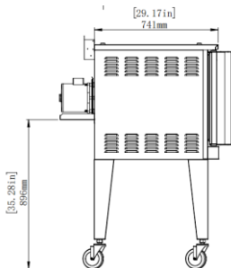
Side dimension chart
