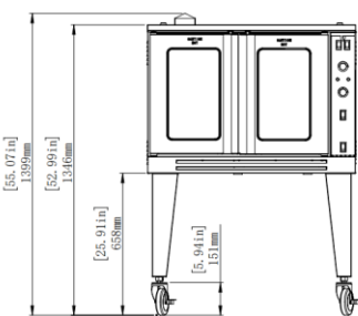
Front dimension chart
