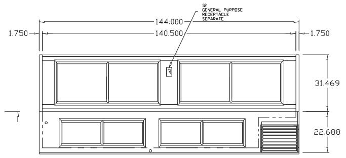
12' REAR VIEW
