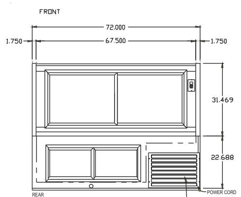
6' REAR VIEW
