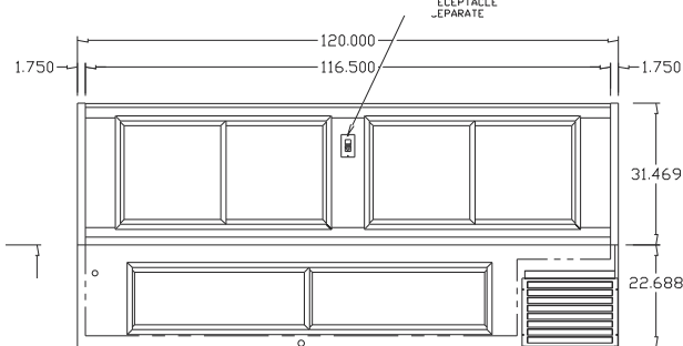
10' REAR VIEW
