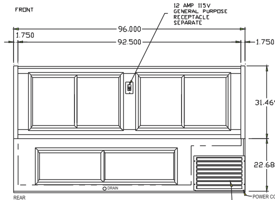
8' REAR VIEW
