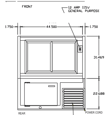
4' REAR VIEW
