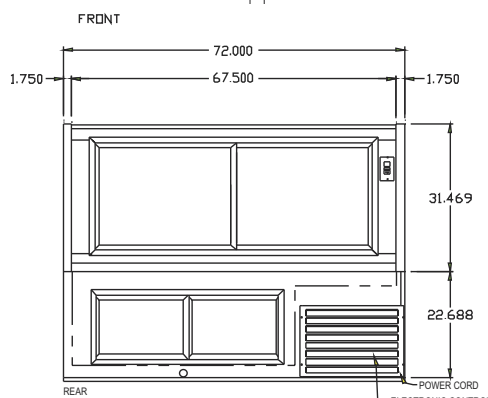
6' REAR VIEW
