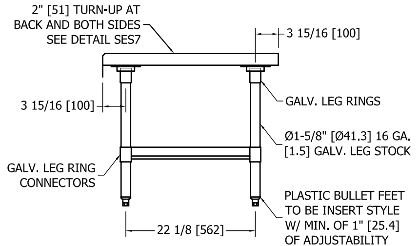
END VIEW
